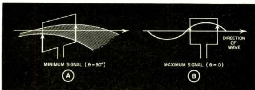
Fig. 3. Manner in which a loop antenna operates
