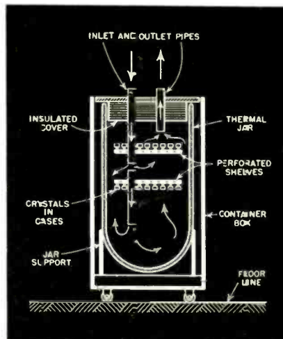
Fig. 3. Details of crystal oven
