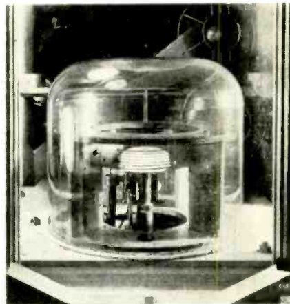
Fig. 2. Hardening a rock bit in an experimental induction furnace
