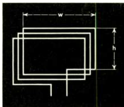
Fig. 2. Diagram of solenoid type loop antenna
