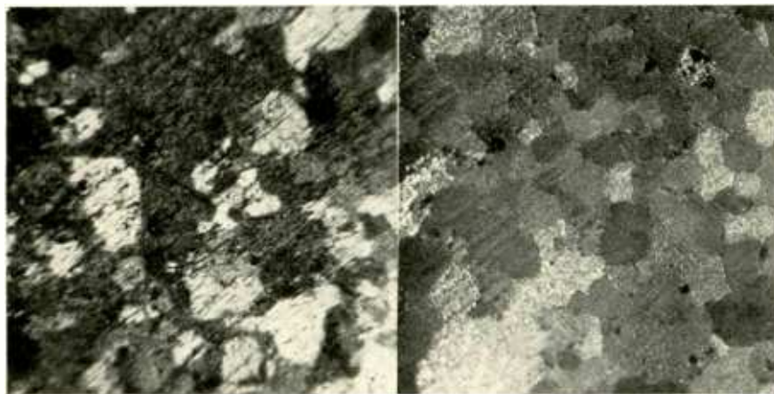
Fig. 3A (left) Photomicrograph of translucent oxide film placed between crossed polaroid discs (mag.=40), and B. (right), etched surface of aluminum foil by reflected light (mag.=75)
